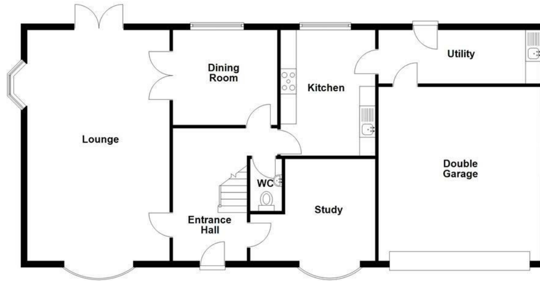
Ground Floor
